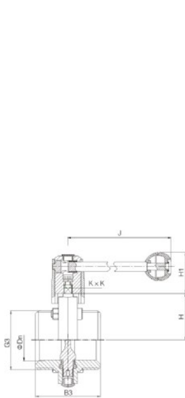
拉式手柄蝶阀 Manual butterfly valve NO.3A-VDF130S1
