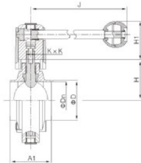
拉动手柄蝶阀 Manual butterfly valve NO.VDF100S1
