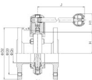
法兰式(圆形) Flange butterfly valve(Round type) NO.VDF240S1
