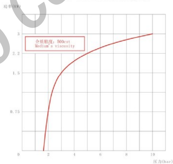
STU-10 压力/功率曲线图 STU-10 pressure/power graph
